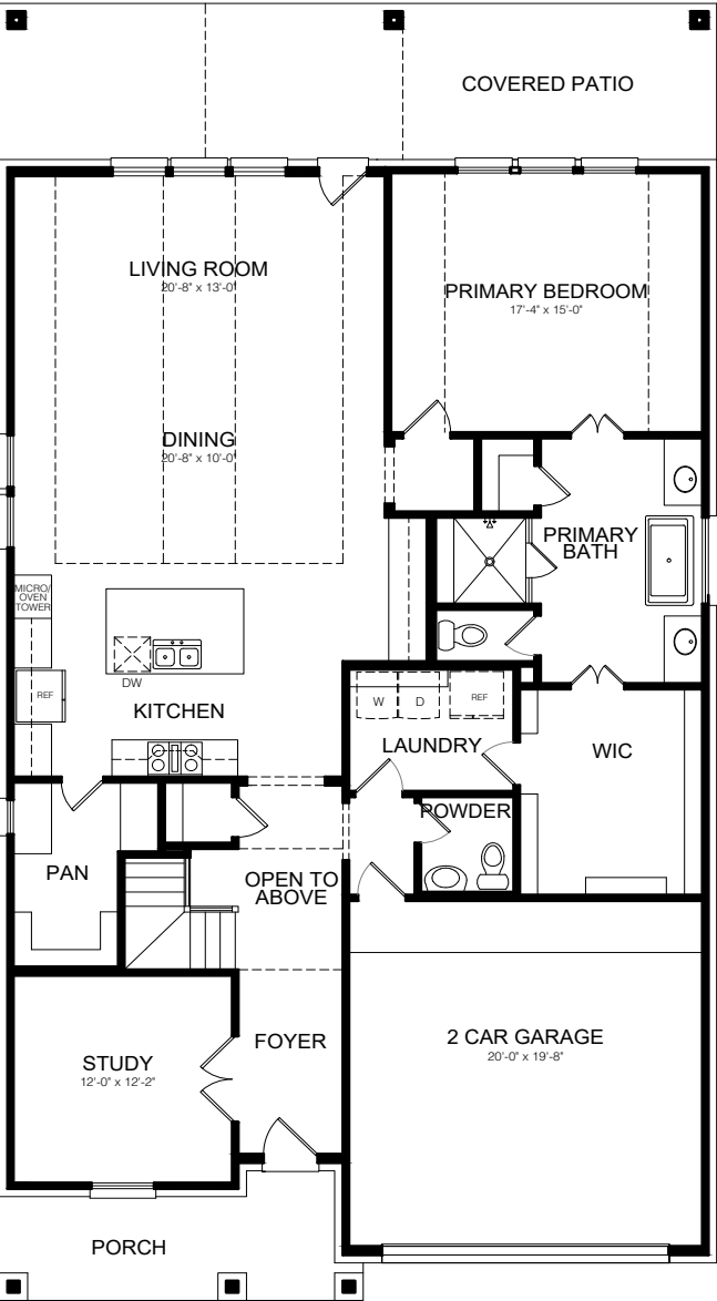
MAIN FLOOR PLAN ELEVATION A
